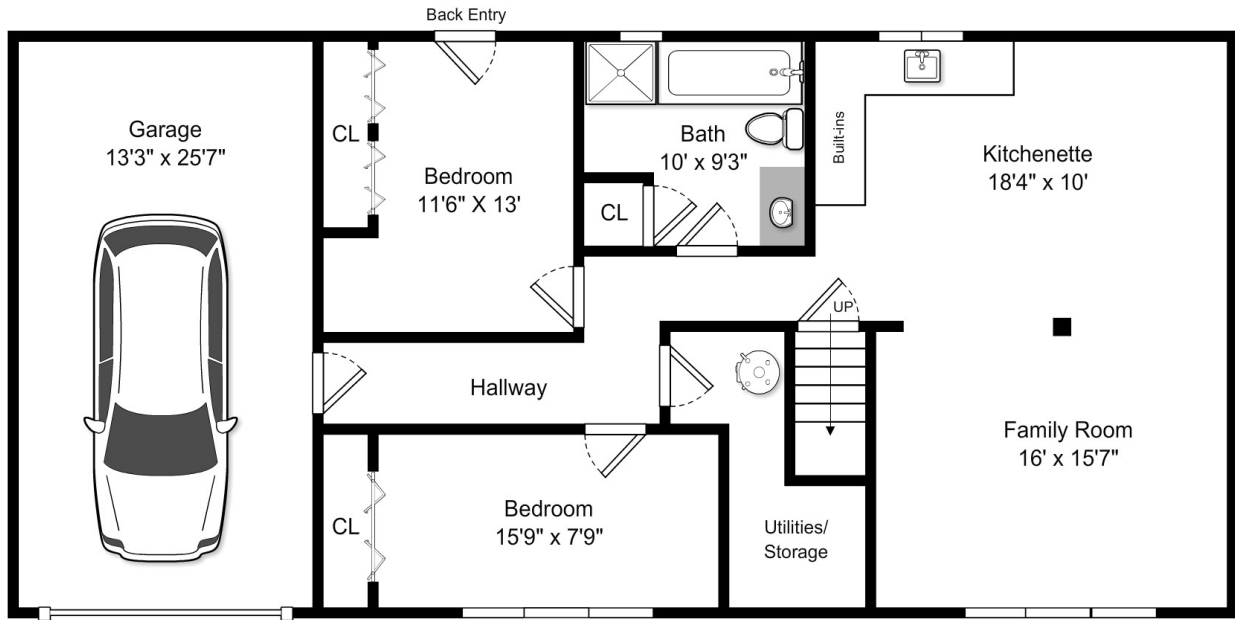
Lower Level
