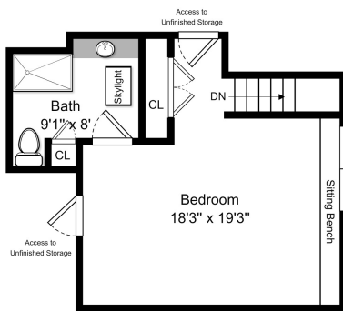
Third Floor
