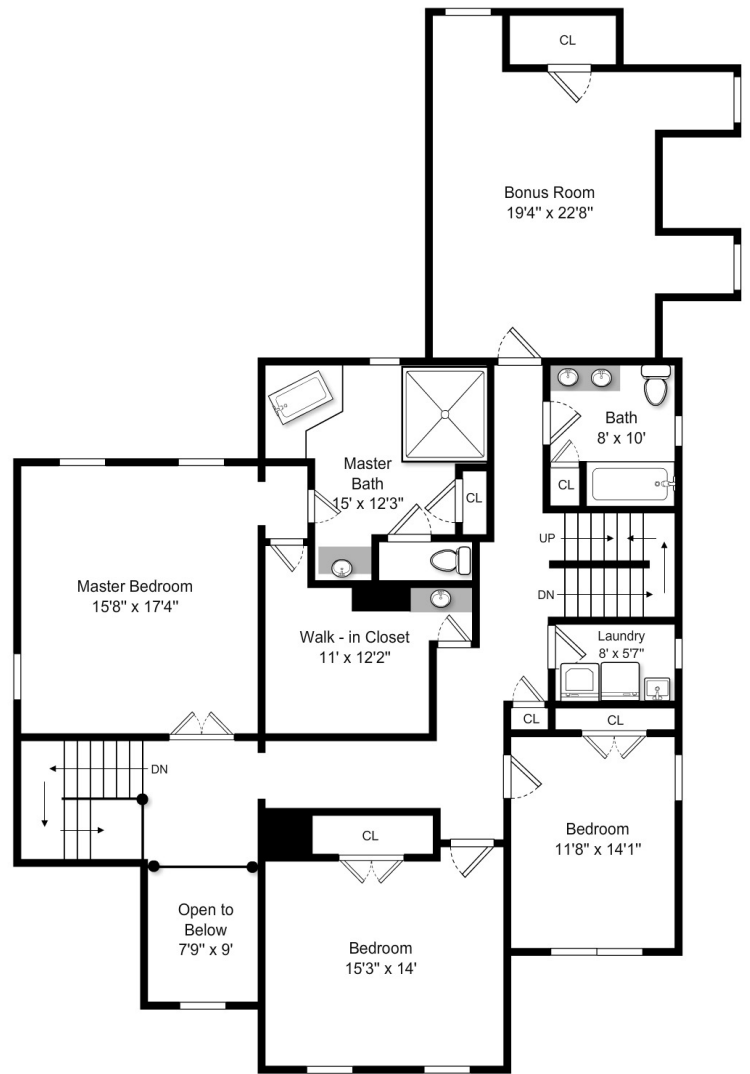
Second Floor
