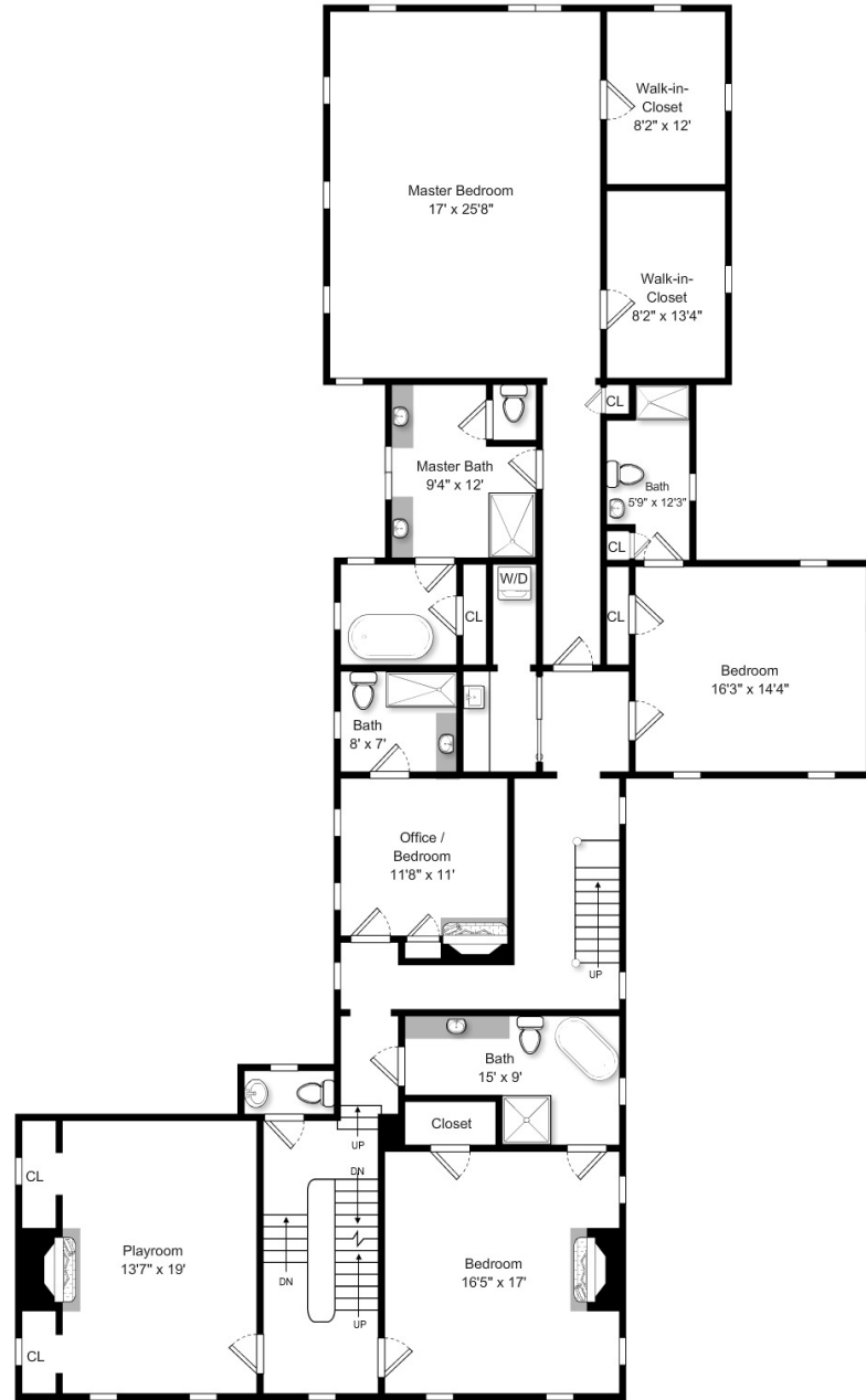
Second Floor
