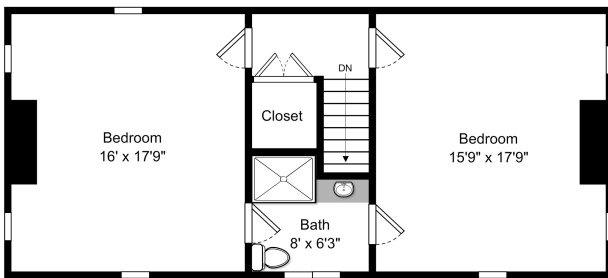
Third Floor
