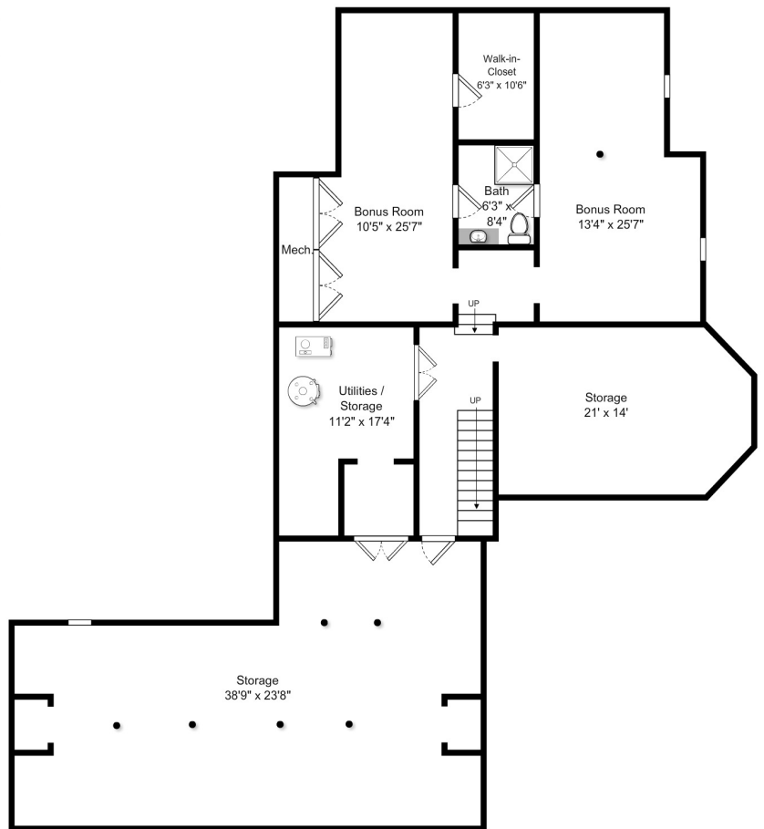
Basement
