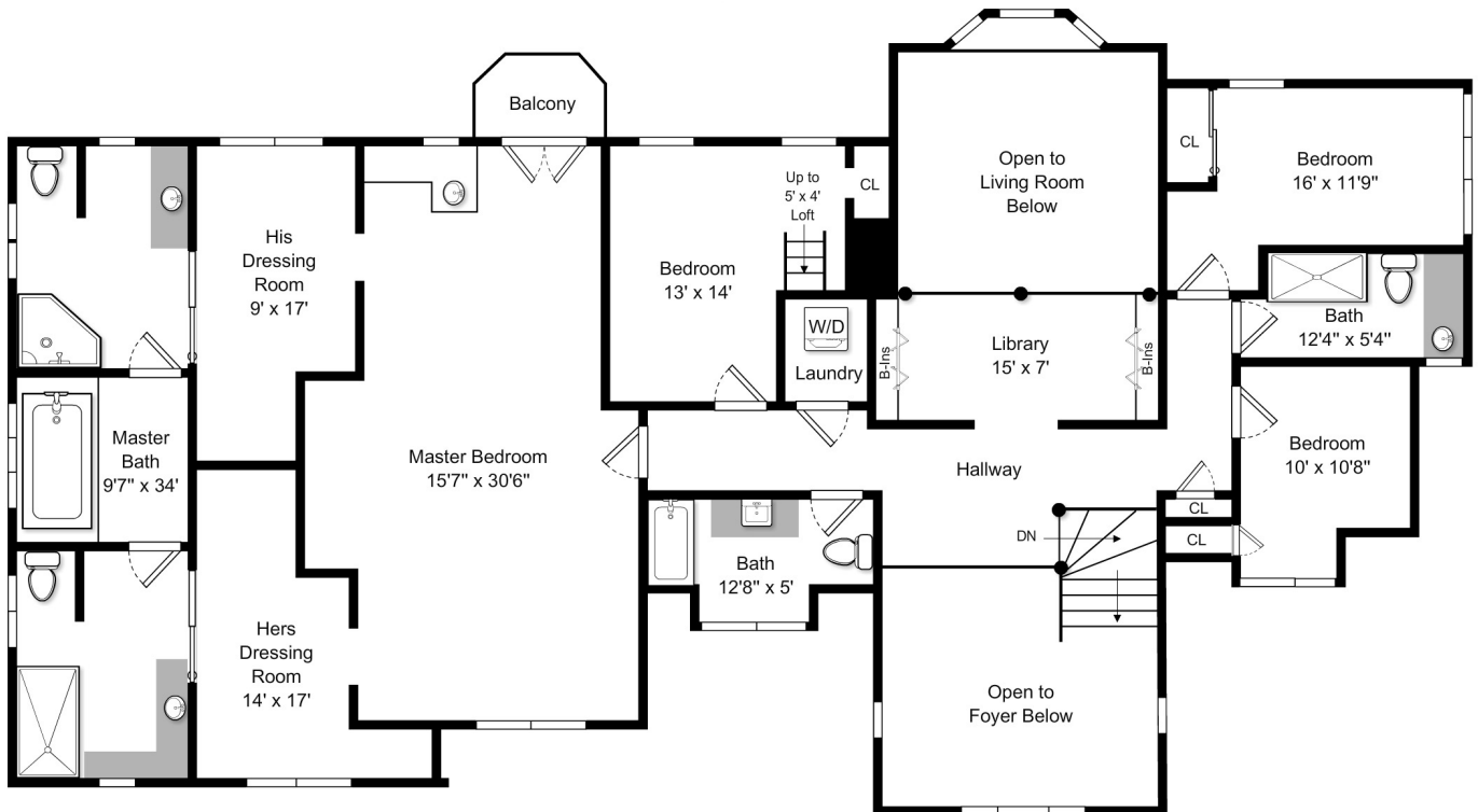
Second Floor
